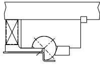
09 = TF PIEGA A "Z" "Z" BEND / "Z" BIEGUNG PLIAGE EN "Z"
